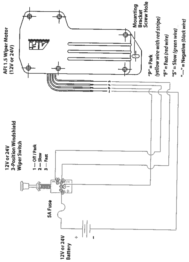
Wiring Diagram #1 (for normal two-speed operation)
